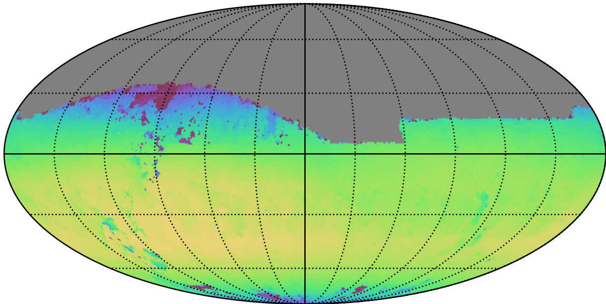
weather_cloudso2v3.4_10yrs Yr 1 i band: Max skyBrightness
