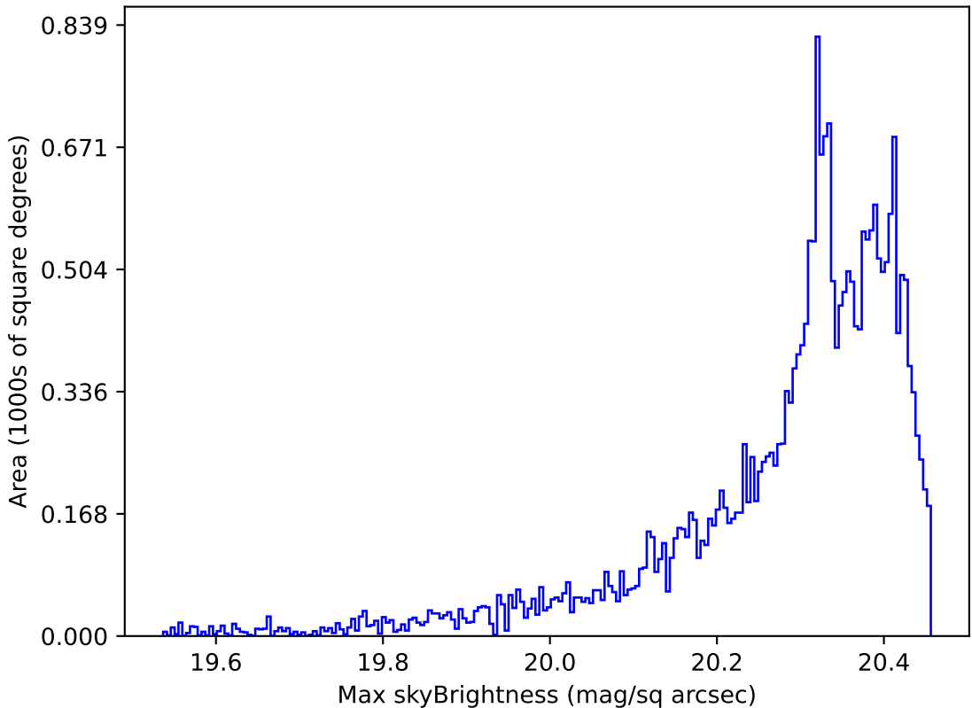
weather_cloudso2v3.4_10yrs Yr 1 i band: Max skyBrightness
