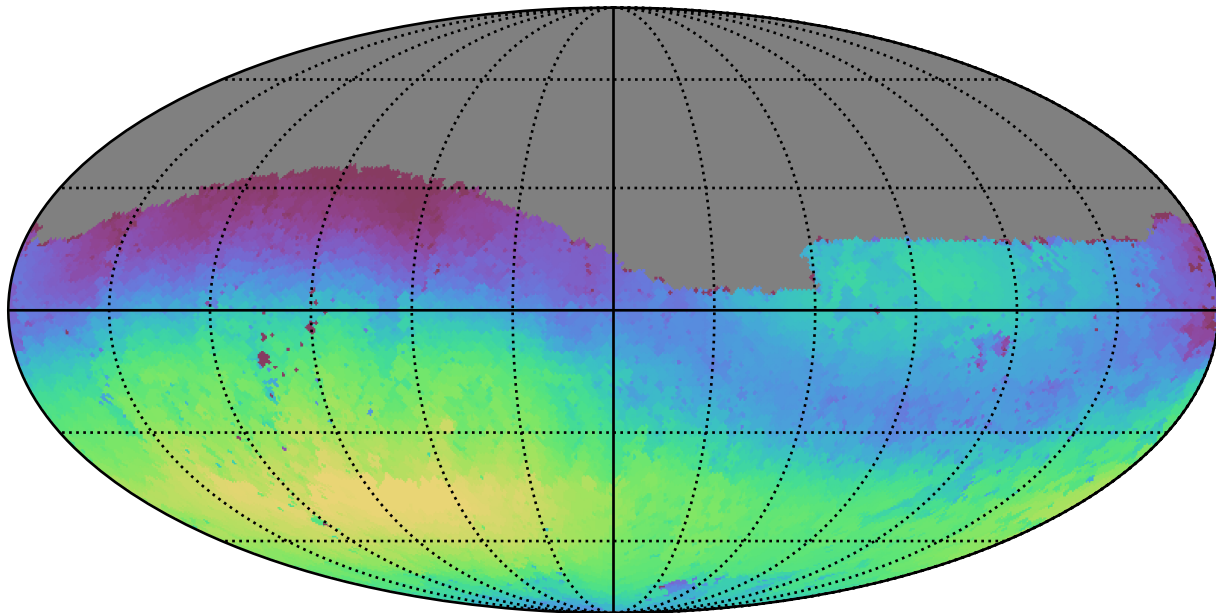
weather_cloudso2v3.4_10yrs Yr 1 g band: Max skyBrightness
