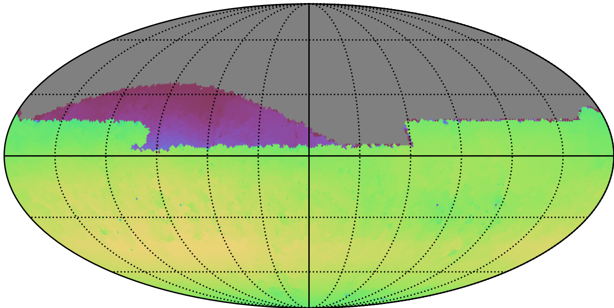
weather_cloudso2v3.4_10yrs Yr1 all bands: Max skyBrightness
