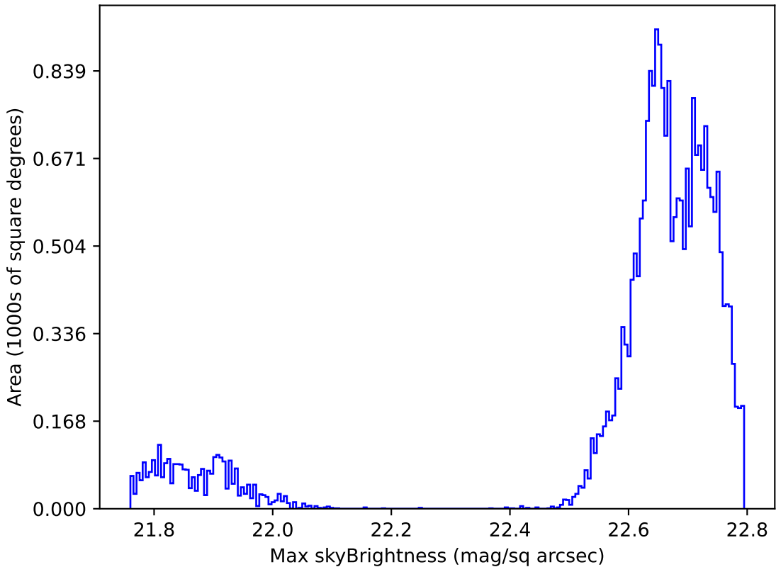
weather_cloudso2v3.4_10yrs Yr 1 all bands: Max skyBrightness
