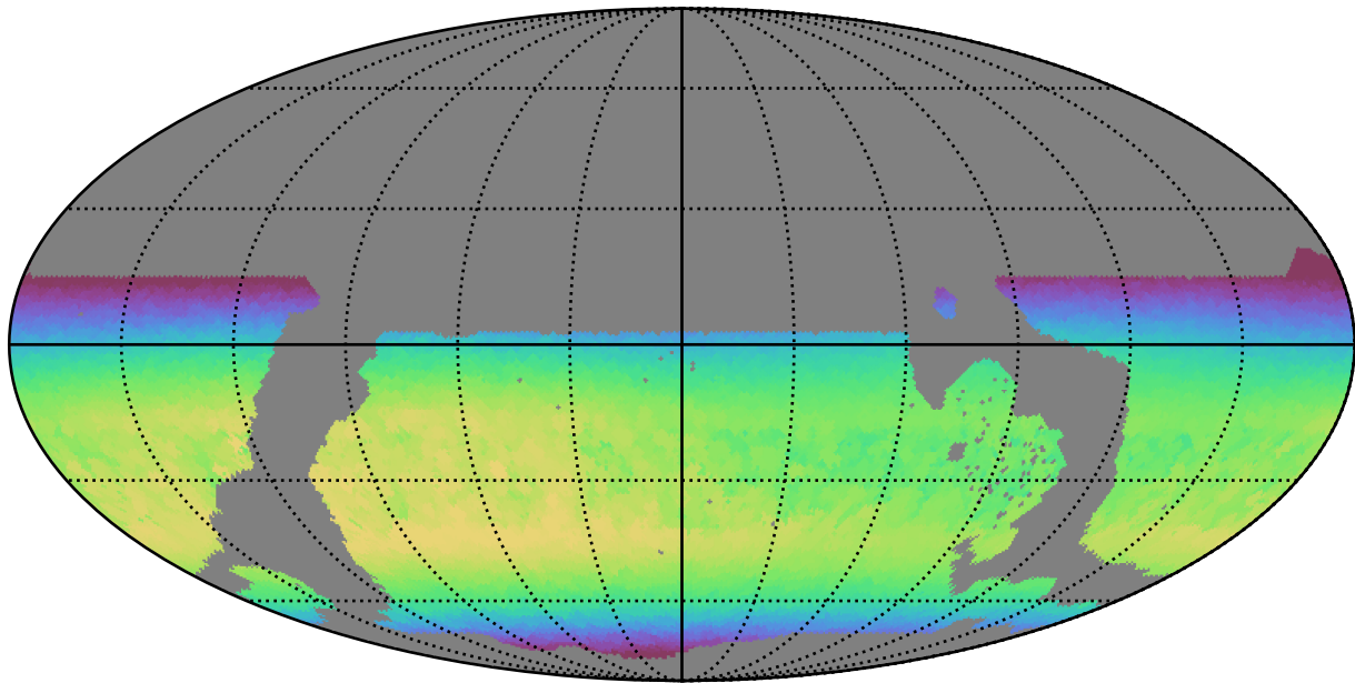
weather_cloudso2v3.4_10yrs WFD z band: Max skyBrightness
