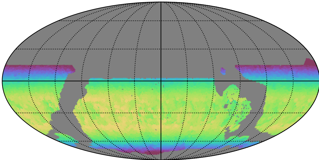
weather_cloudso2v3.4_10yrs WFD y band: Max skyBrightness
