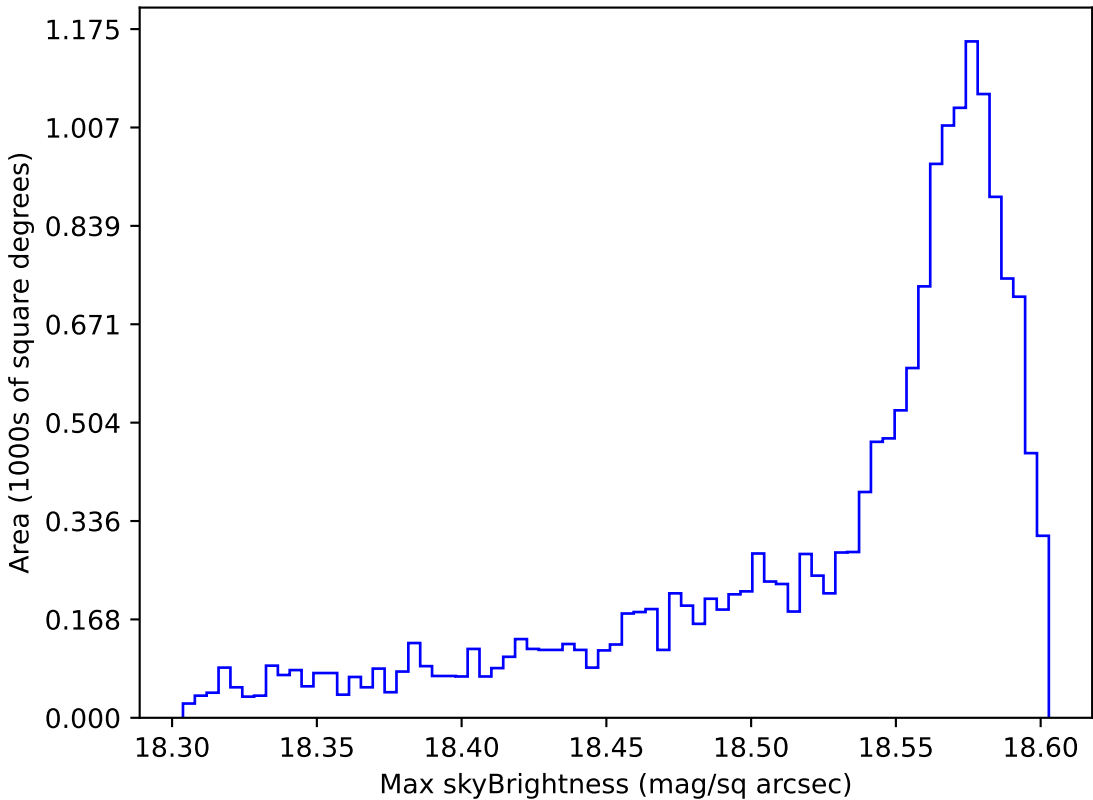
weather_cloudso2v3.4_10yrs WFD y band: Max skyBrightness
