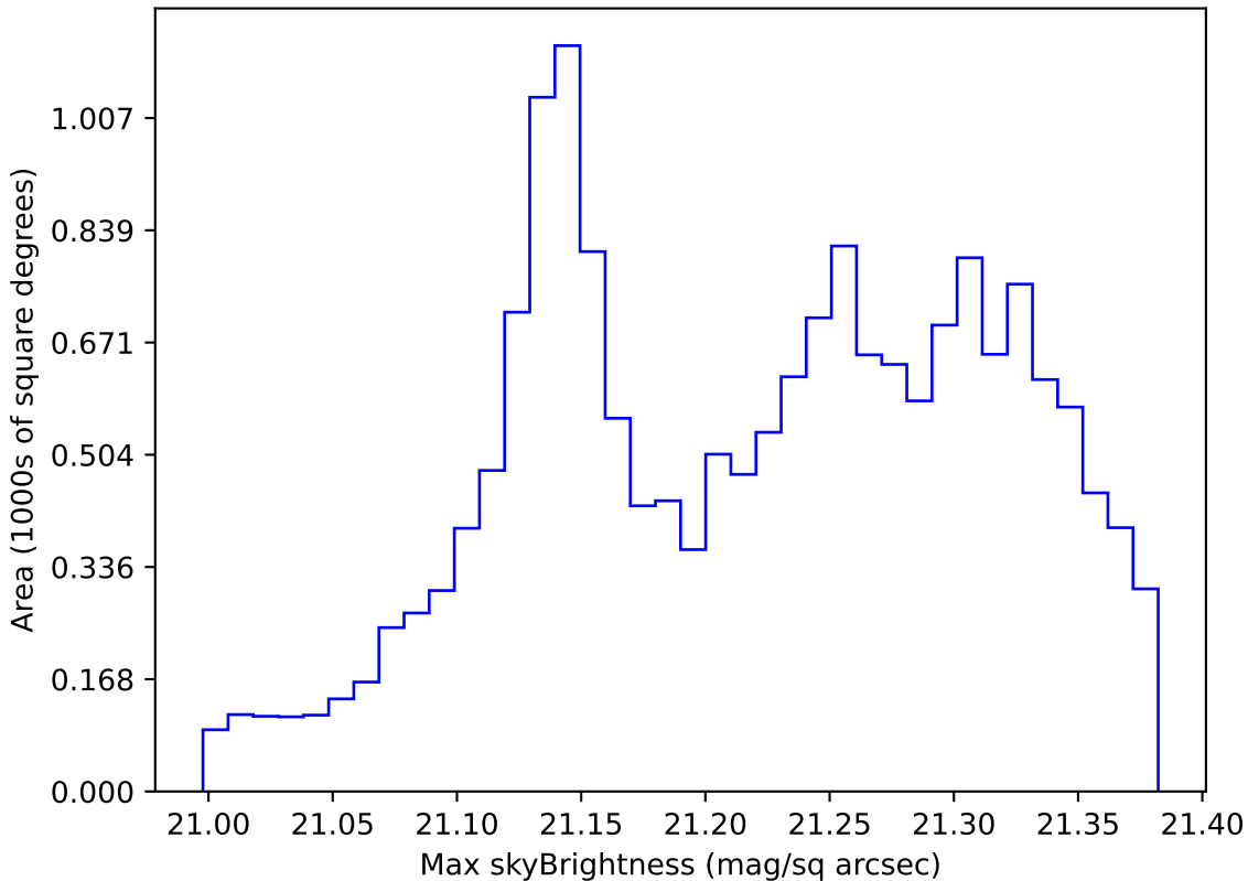
weather_cloudso2v3.4_10yrs WFD r band: Max skyBrightness
