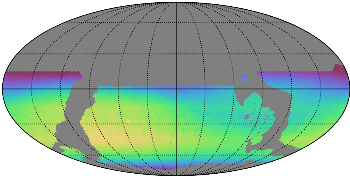
weather_cloudso2v3.4_10yrs WFD i band: Max skyBrightness
