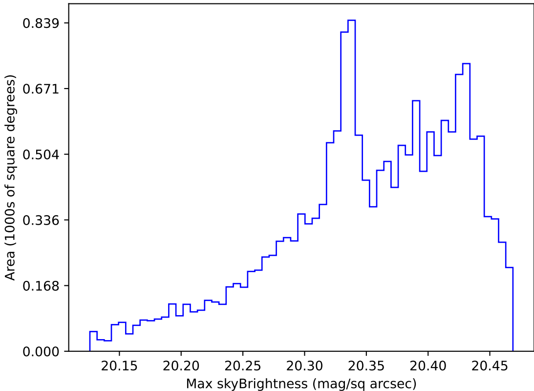
weather_cloudso2v3.4_10yrs WFD i band: Max skyBrightness
