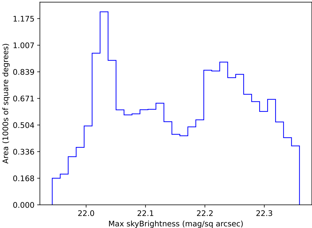
weather_cloudso2v3.4_10yrs WFD g band: Max skyBrightness
