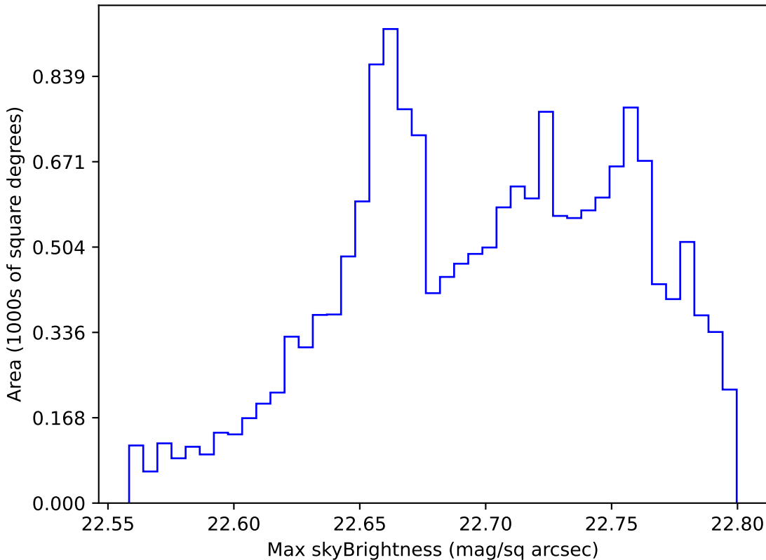
weather_cloudso2v3.4_10yrs WFD all bands: Max skyBrightness
