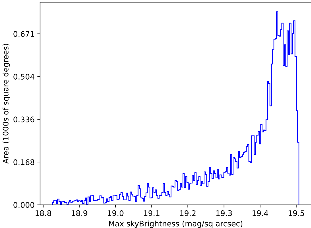
weather_cloudso2v3.4_10yrs All sky z band: Max skyBrightness
