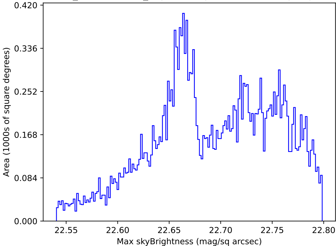
weather_cloudso2v3.4_10yrs All sky u band: Max skyBrightness
