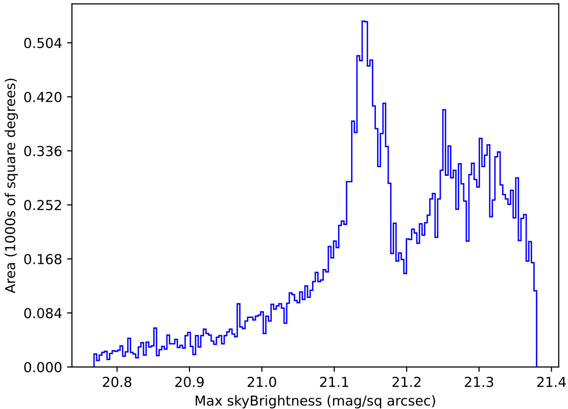
weather_cloudso2v3.4_10yrs All sky r band: Max skyBrightness
