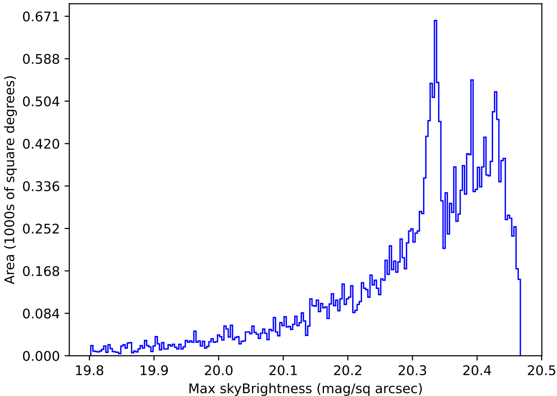
weather_cloudso2v3.4_10yrs All sky i band: Max skyBrightness
