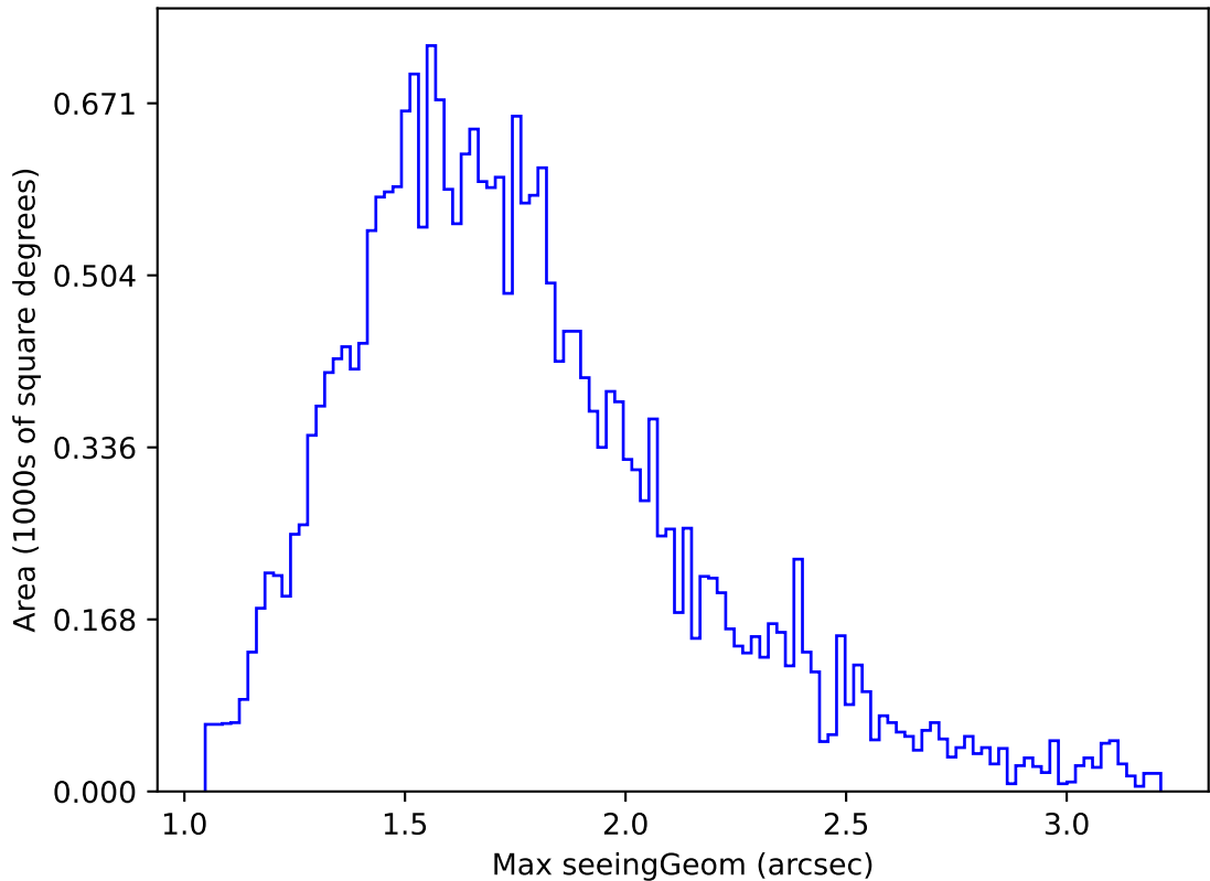
weather_cloudso2v3.4_10yrs Yr 1 all bands: Max seeingGeom
