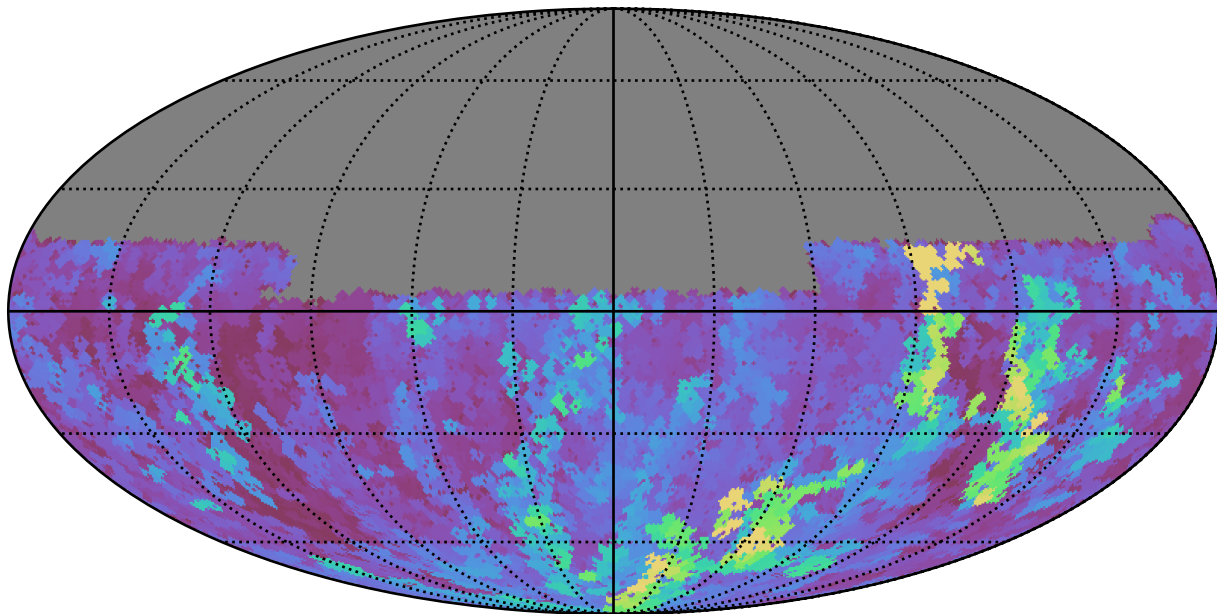
weather_cloudso2v3.4_10yrs Yr 1 u band: Max seeingEff
