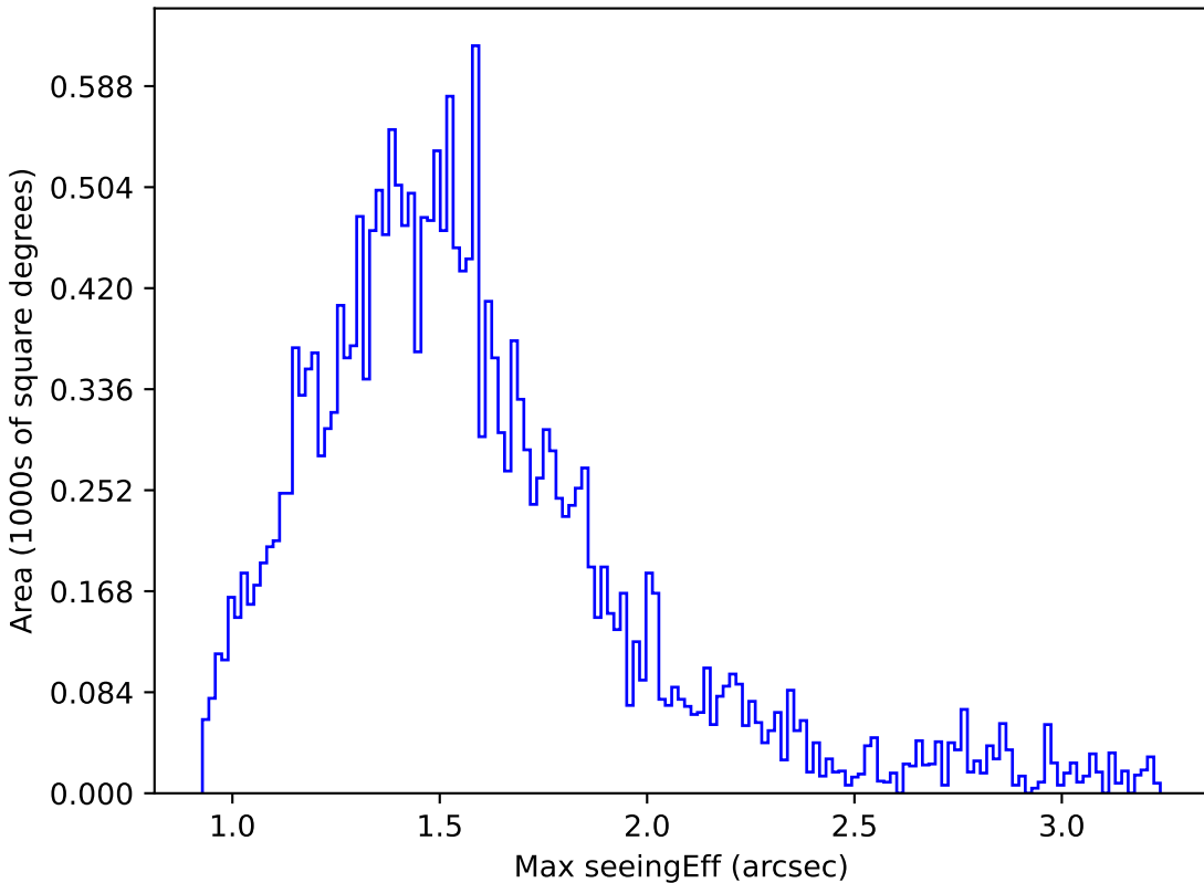
weather_cloudso2v3.4_10yrs Yr 1 u band: Max seeingEff
