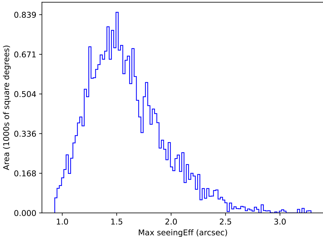
weather_cloudso2v3.4_10yrs Yr 1 r band: Max seeingEff
