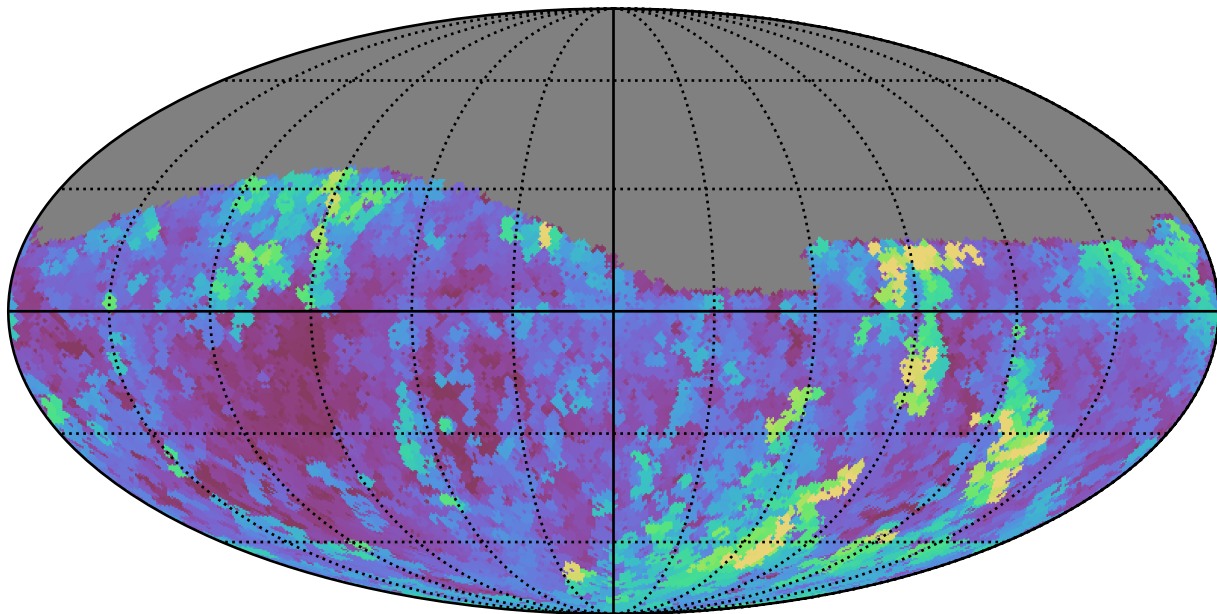
weather_cloudso2v3.4_10yrs Yr 1 g band: Max seeingEff
