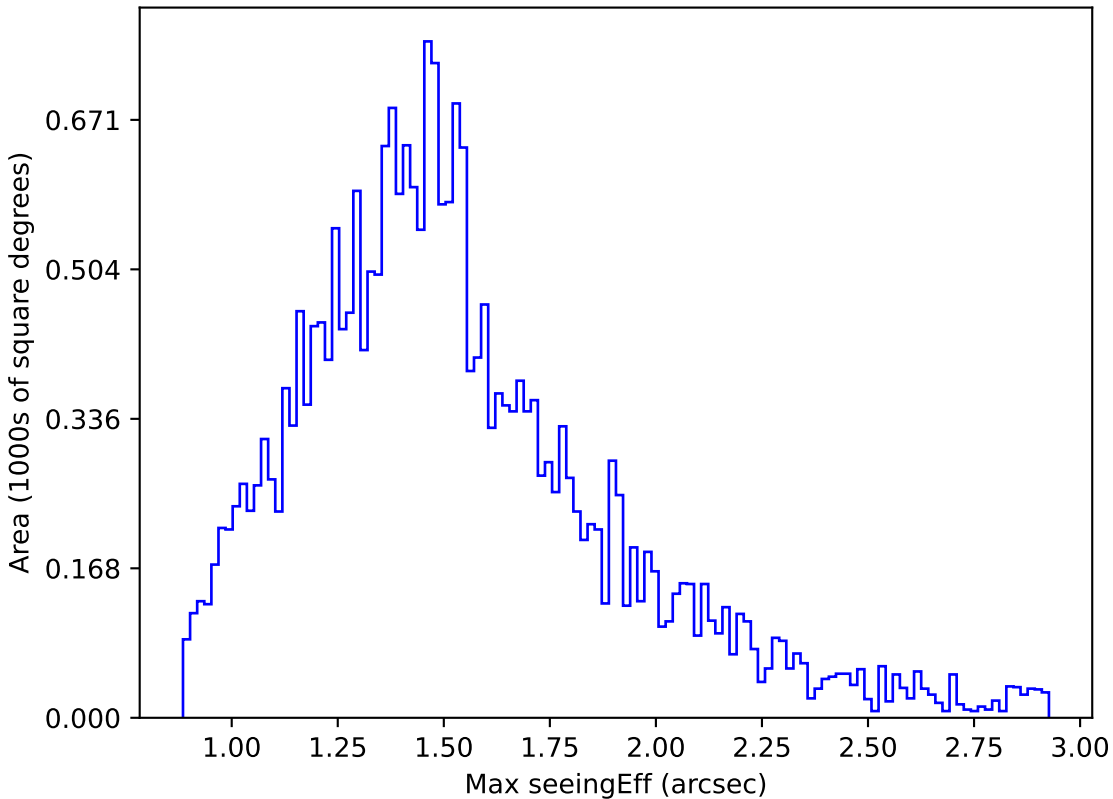
weather_cloudso2v3.4_10yrs Yr 1 g band: Max seeingEff
