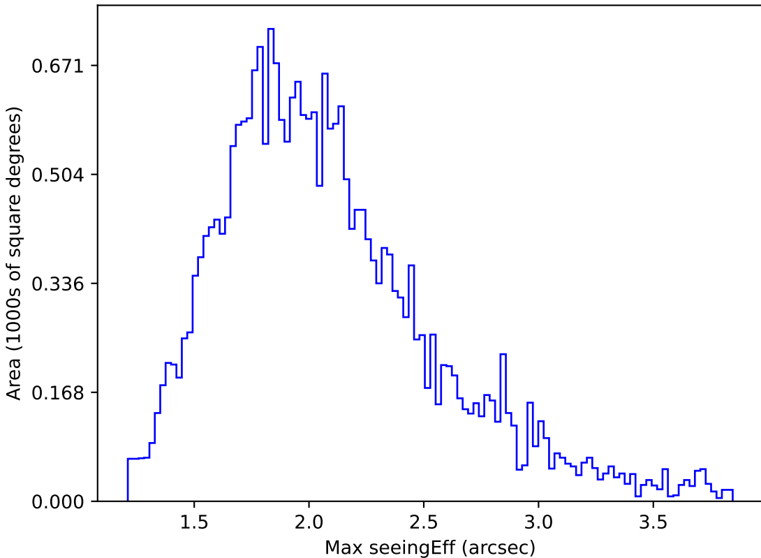
weather_cloudso2v3.4_10yrs Yr 1 all bands: Max seeingEff
