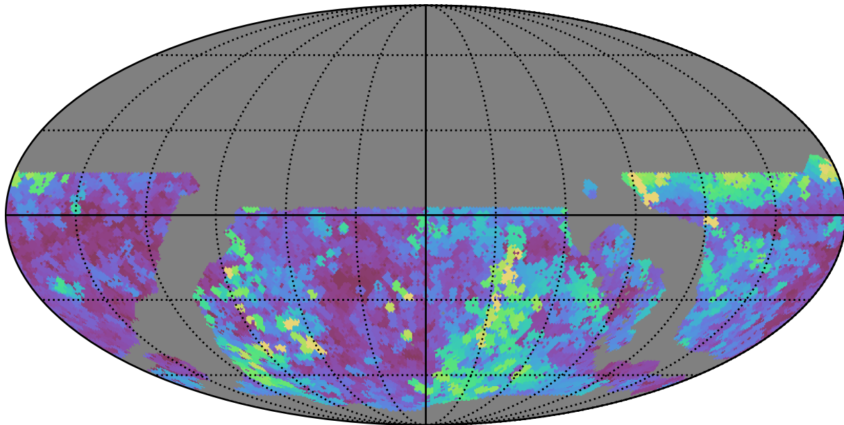
weather_cloudso2v3.4_10yrs WFD u band: Max seeingEff
