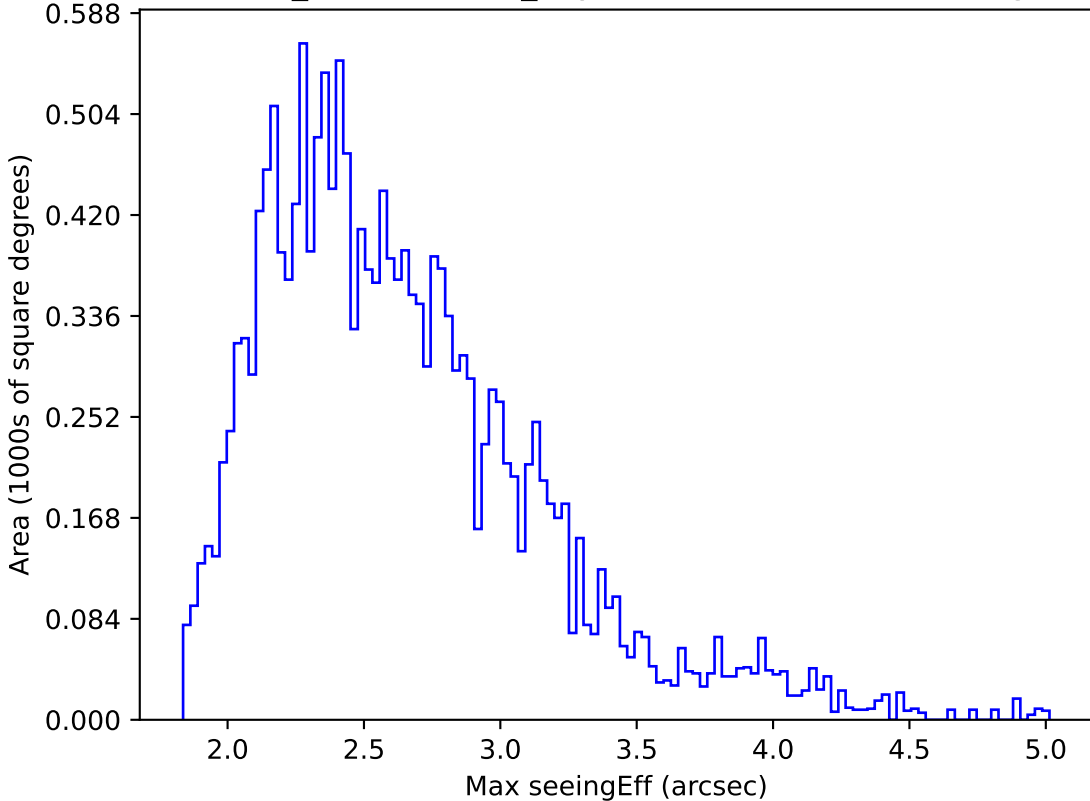
weather_cloudso2v3.4_10yrs WFD r band: Max seeingEff
