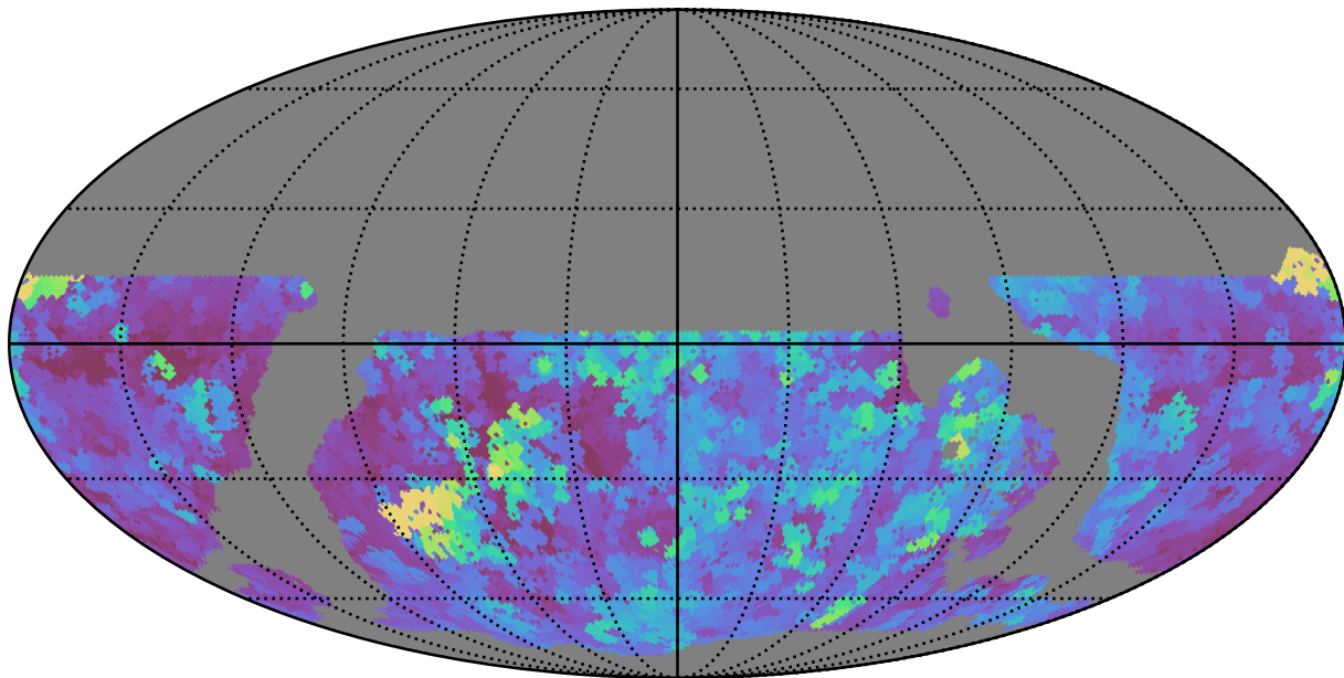
weather_cloudso2v3.4_10yrs WFD g band: Max seeingEff
