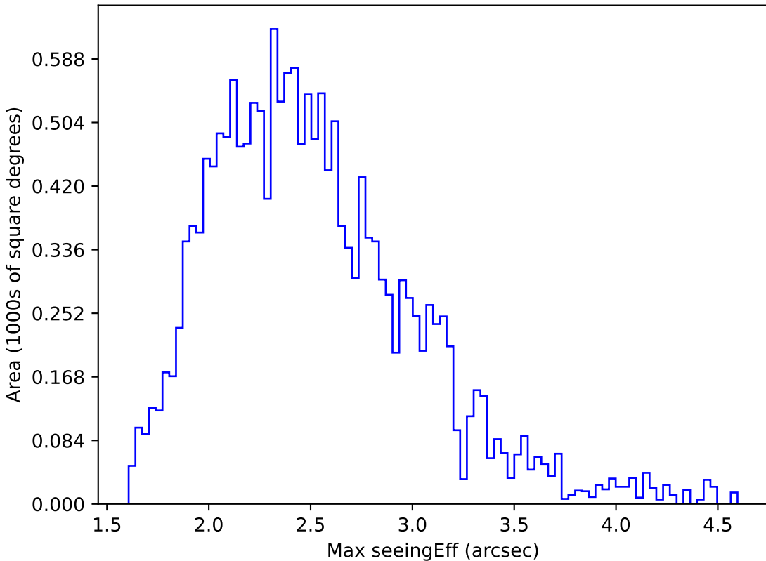
weather_cloudso2v3.4_10yrs WFD g band: Max seeingEff
