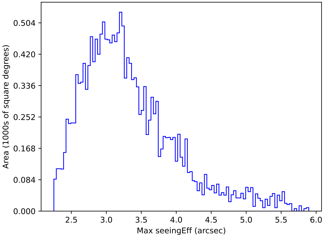
weather_cloudso2v3.4_10yrs WFD all bands: Max seeingEff
