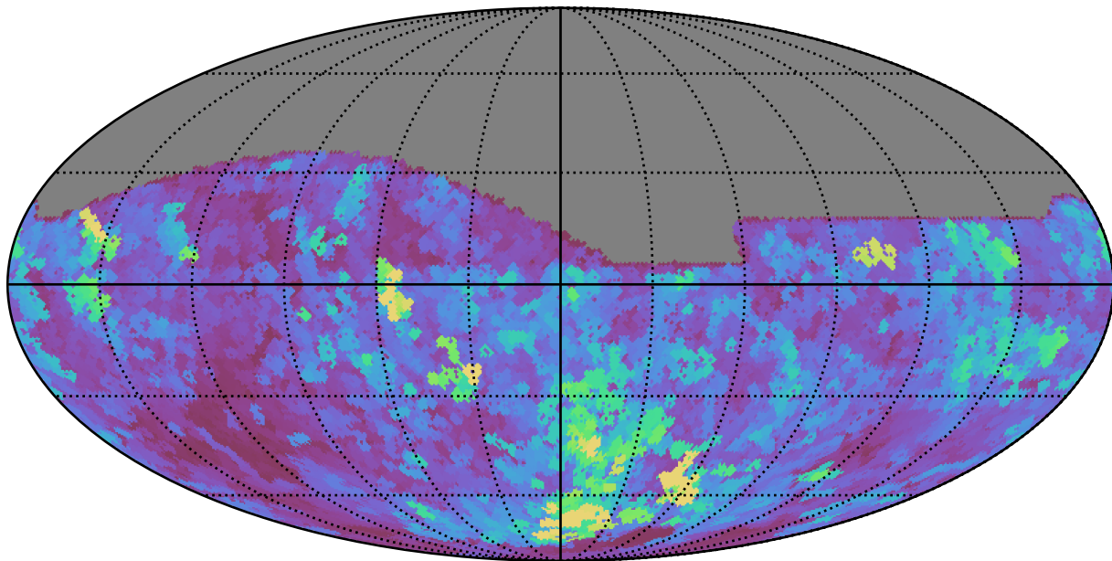
weather_cloudso2v3.4_10yrs All sky z band: Max seeingEff
