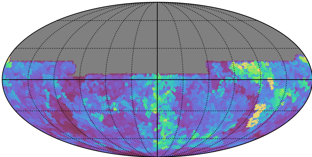
weather_cloudso2v3.4_10yrs All sky y band: Max seeingEff
