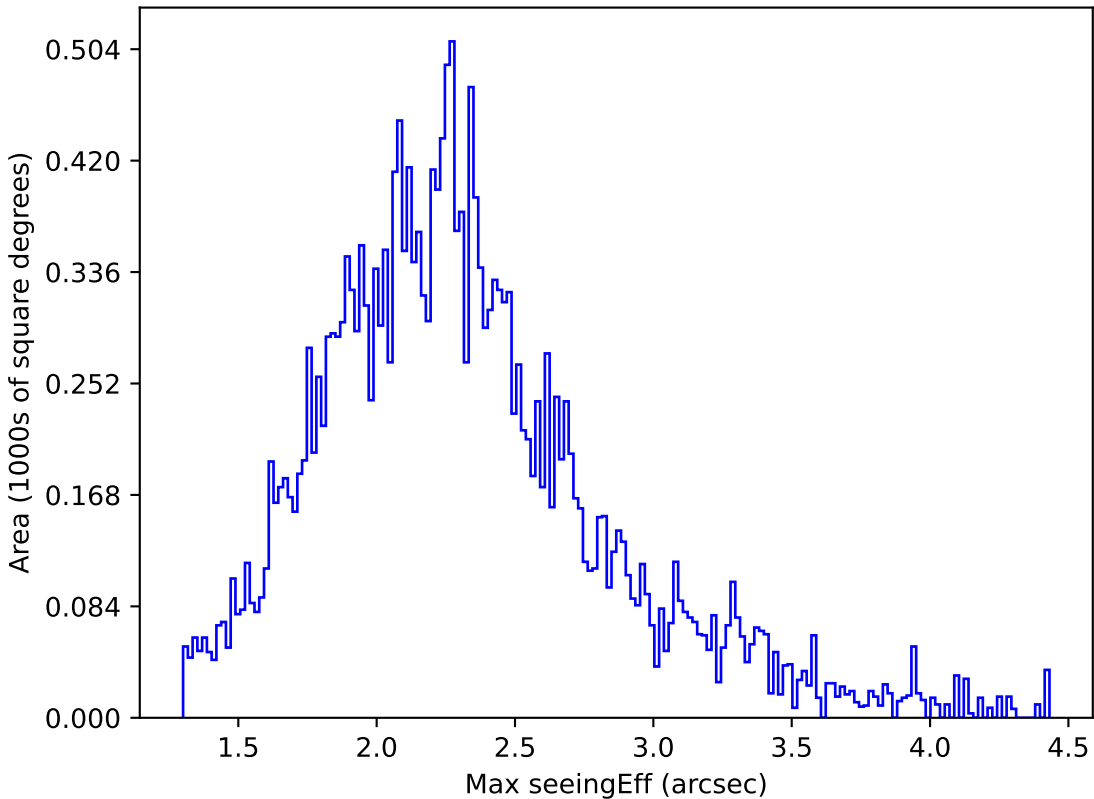
weather_cloudso2v3.4_10yrs All sky y band: Max seeingEff
