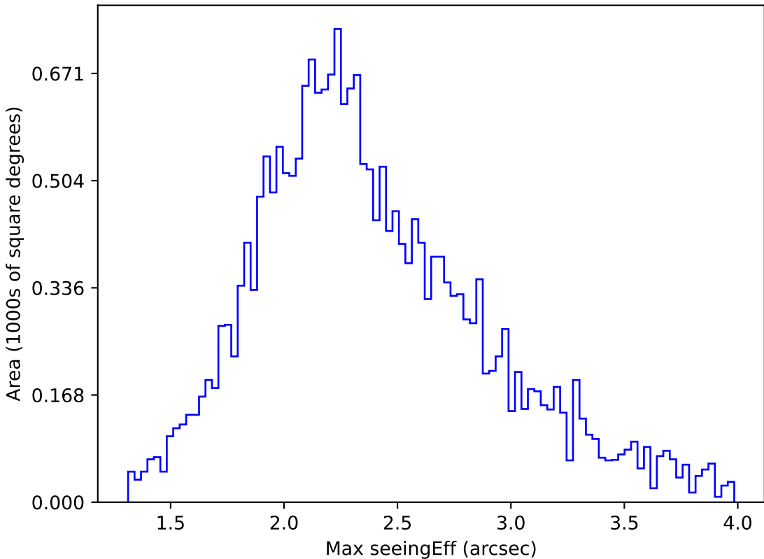
weather_cloudso2v3.4_10yrs All sky u band: Max seeingEff
