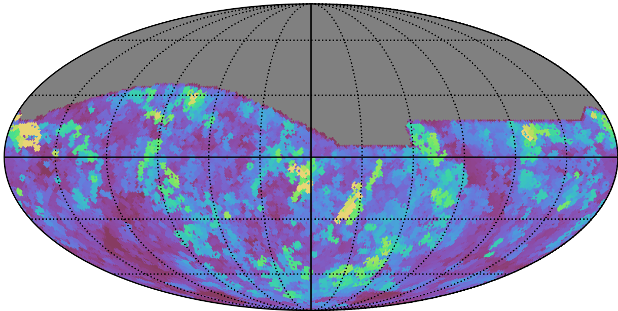
weather_cloudso2v3.4_10yrs All sky r band: Max seeingEff
