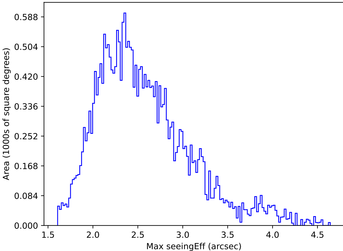
weather_cloudso2v3.4_10yrs All sky r band: Max seeingEff
