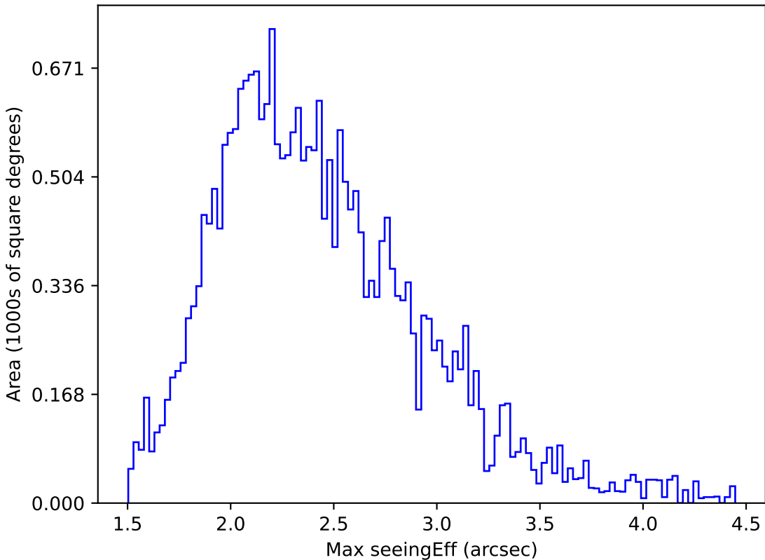
weather_cloudso2v3.4_10yrs All sky g band: Max seeingEff
