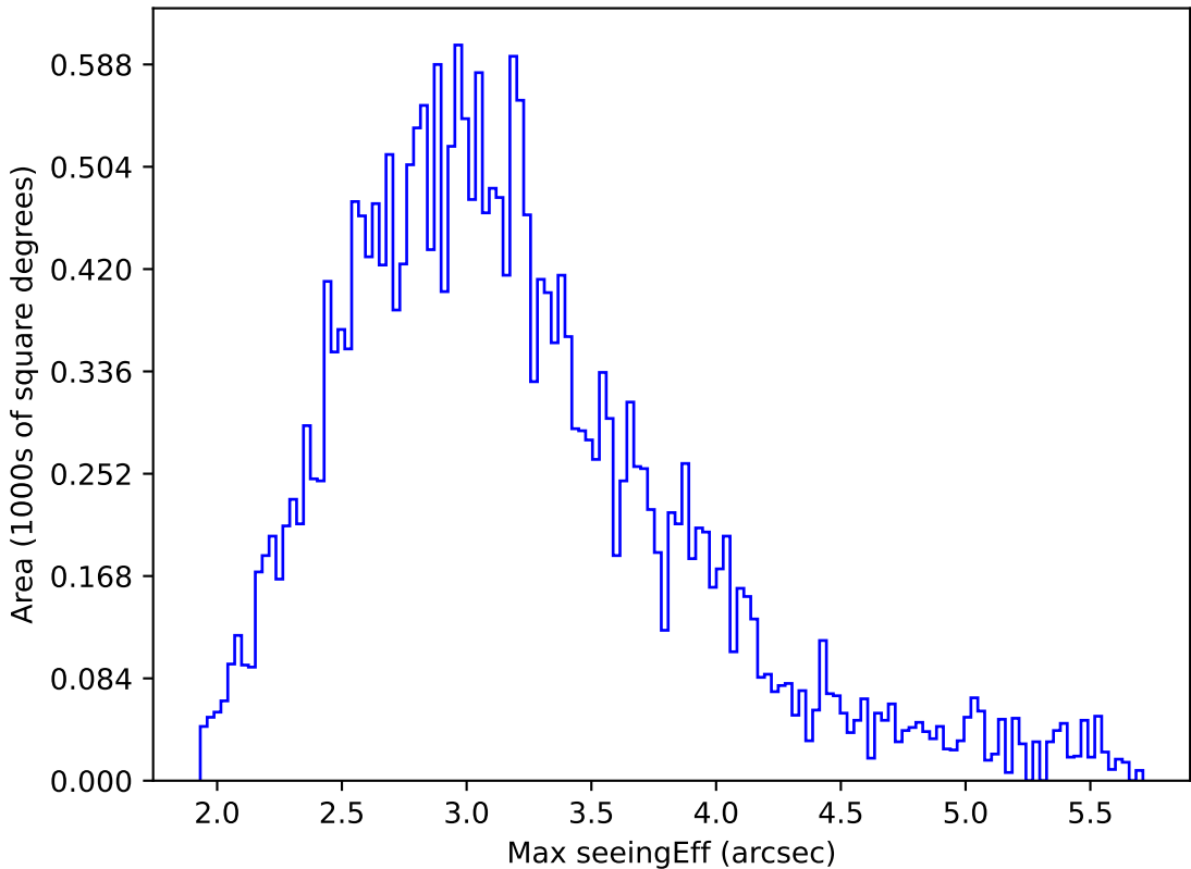
weather_cloudso2v3.4_10yrs All sky all bands: Max seeingEff
