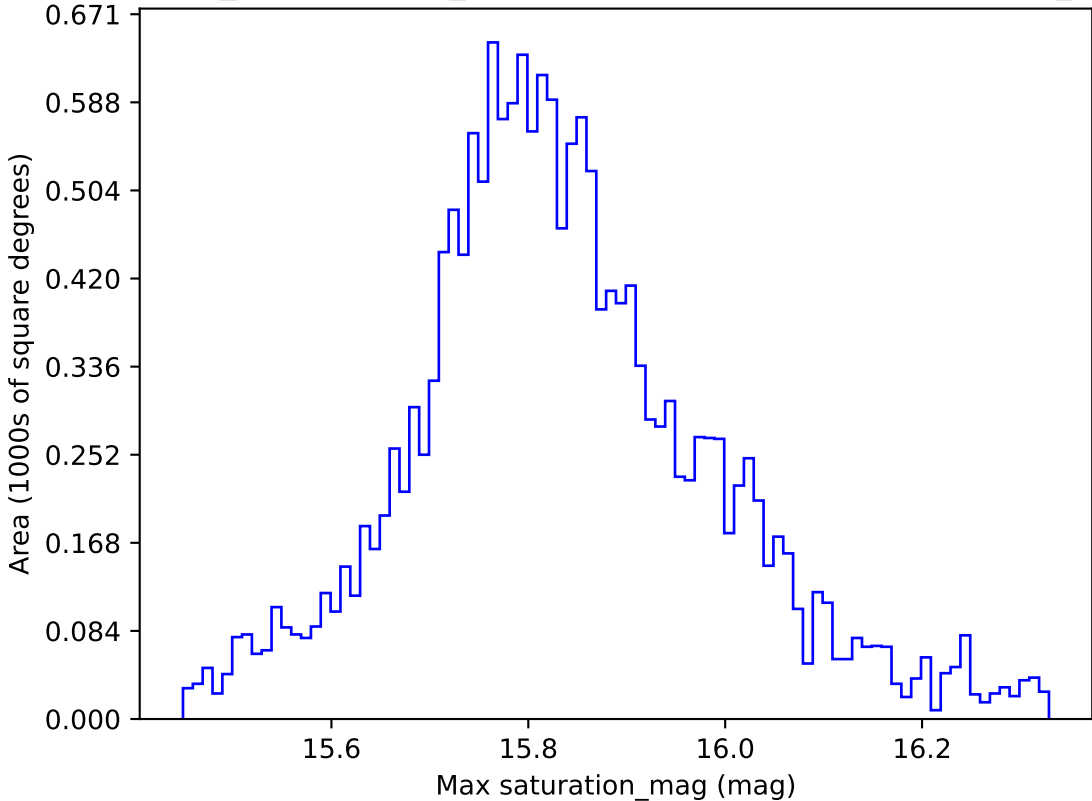
weather_cloudso2v3.4_10yrs WFD all bands: Max saturation_mag
