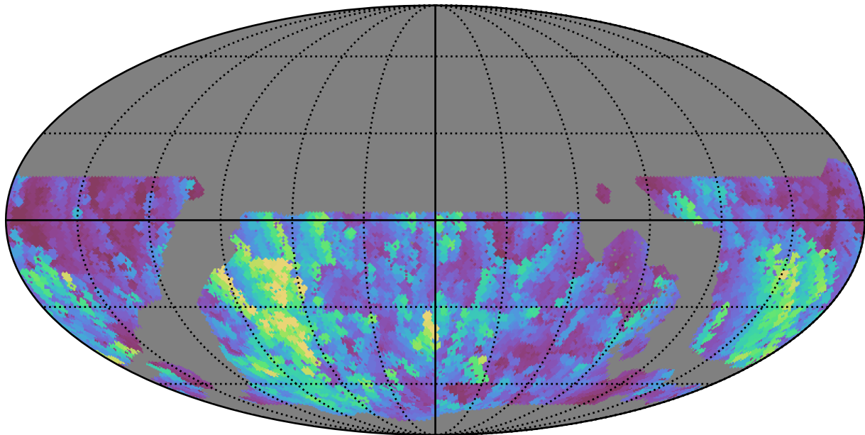
weather_cloudso2v3.4_10yrs WFD u band: Max normairmass
