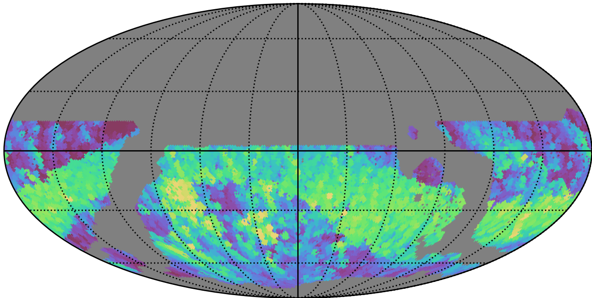
weather_cloudso2v3.4_10yrs WFD r band: Max normairmass
