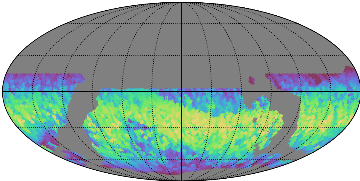
weather_cloudso2v3.4_10yrs WFD all bands: Max normairmass
