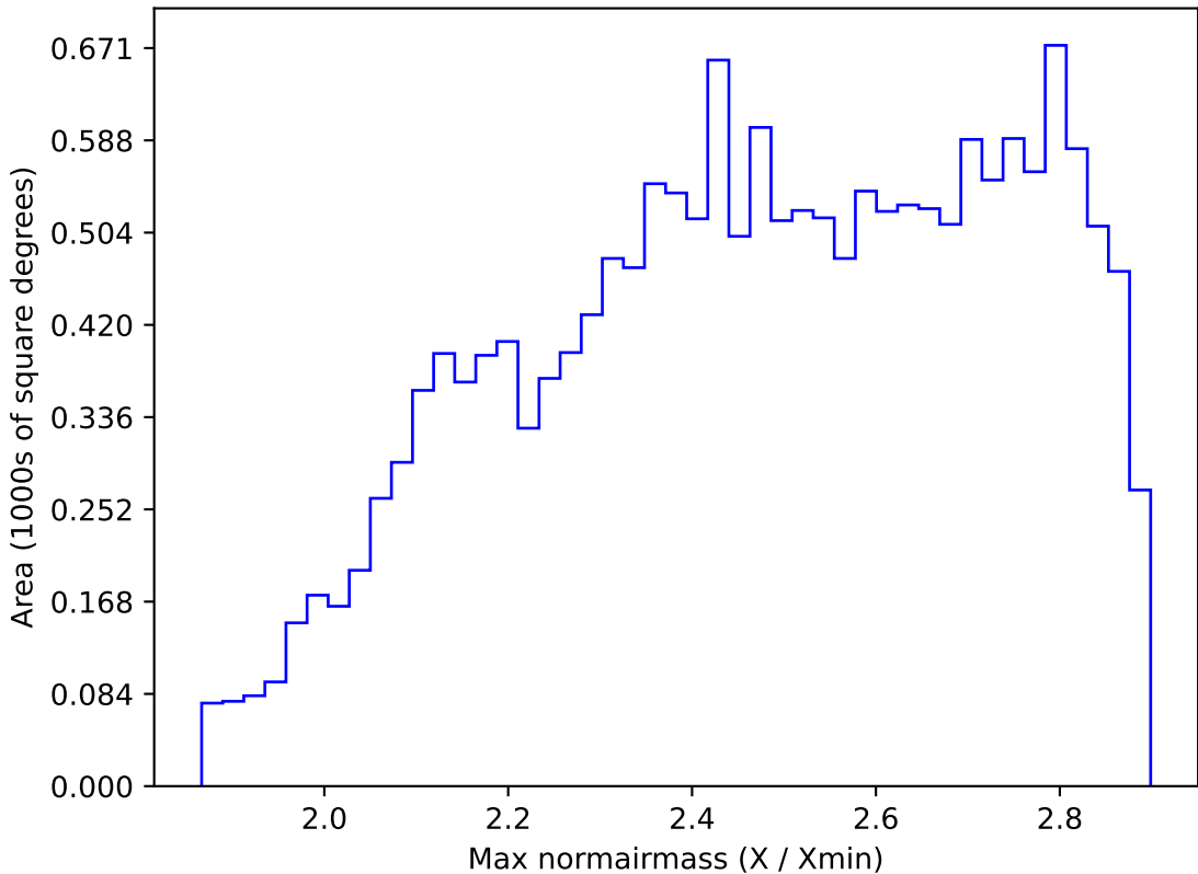
weather_cloudso2v3.4_10yrs WFD all bands: Max normairmass
