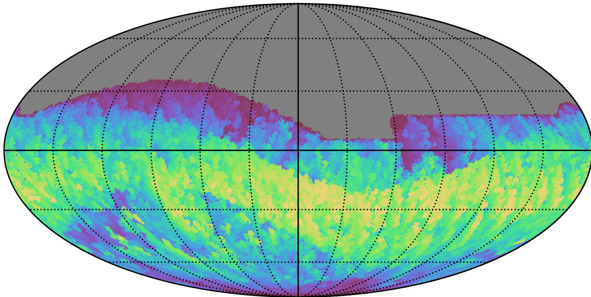
weather_cloudso2v3.4_10yrs All sky z band: Max normairmass
