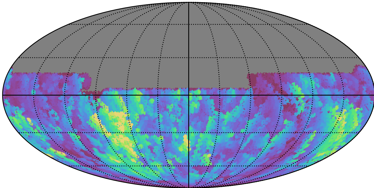
weather_cloudso2v3.4_10yrs All sky u band: Max normairmass
