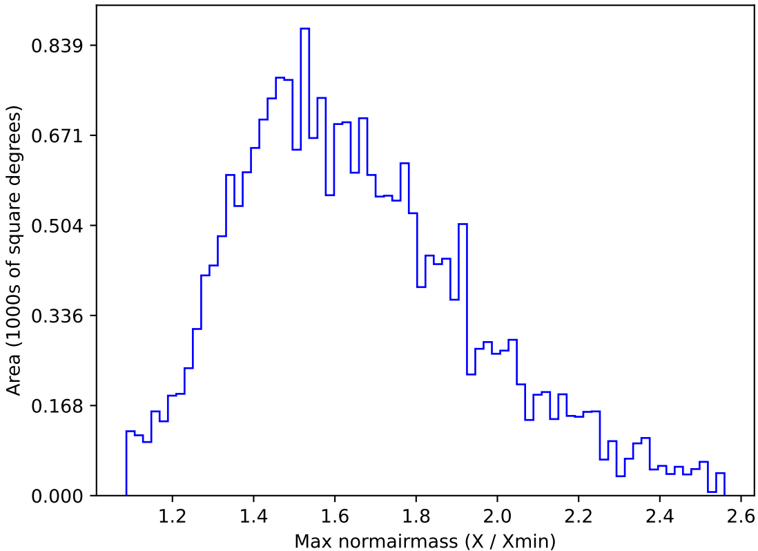
weather_cloudso2v3.4_10yrs All sky u band: Max normairmass
