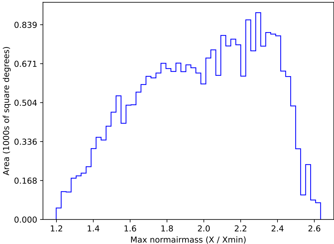
weather_cloudso2v3.4_10yrs All sky r band: Max normairmass
