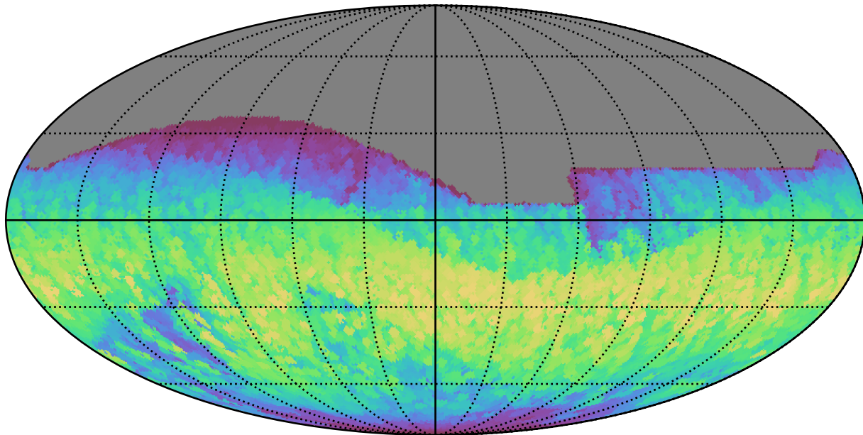
weather_cloudso2v3.4_10yrs All sky all bands: Max normairmass
