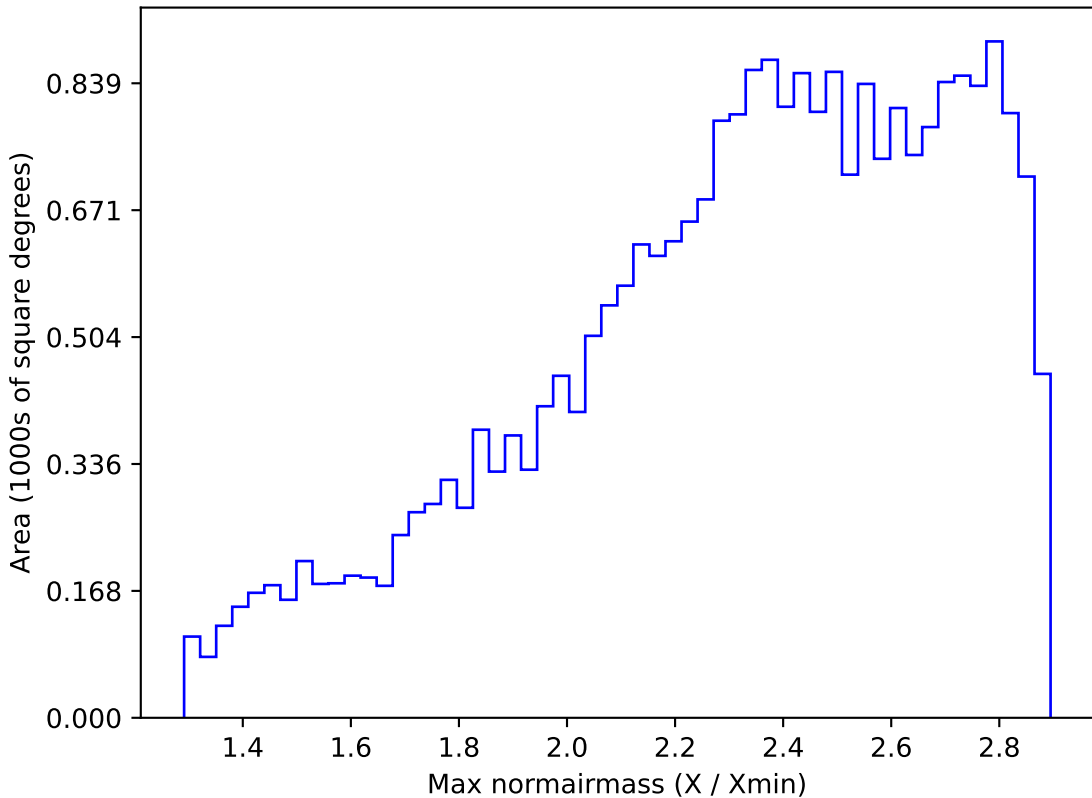
weather_cloudso2v3.4_10yrs All sky all bands: Max normairmass
