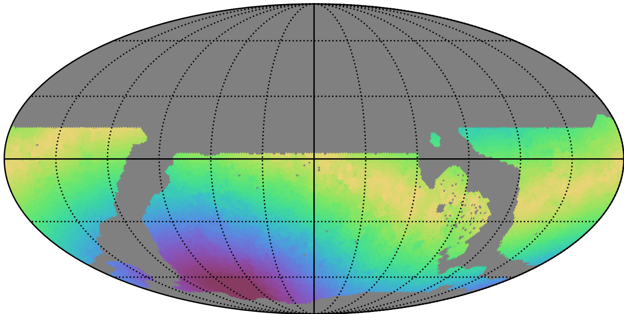
weather_cloudso2v3.4_10yrs WFD u band: Max moonDistance
