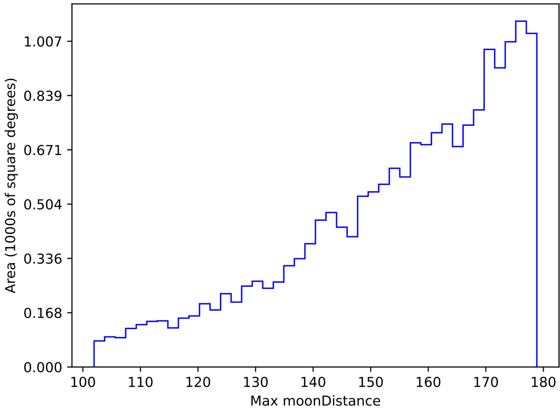
weather_cloudso2v3.4_10yrs WFD u band: Max moonDistance
